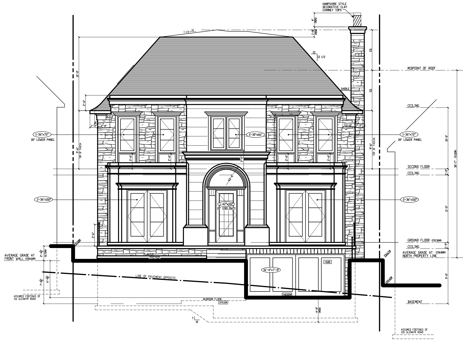
EAST ELEVATION
